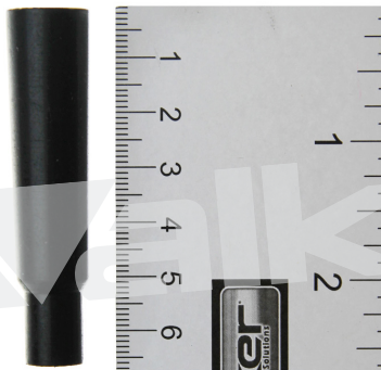
BOT6562 180° Spark Plug Boot
