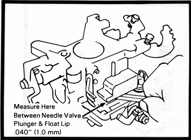
Measuring Float Clearance
