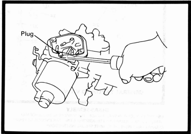
Removing Suction Chamber Adjusting Pin
