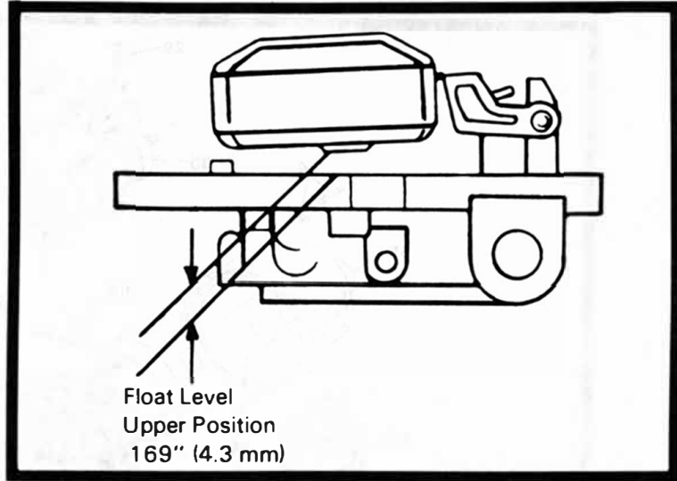
Measuring Float Drop
