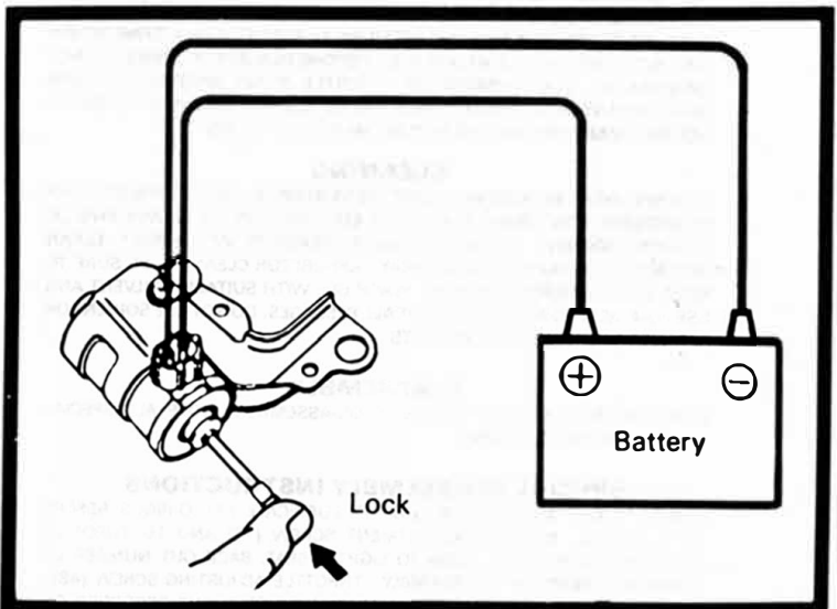
Checking Throttle Valve Solenoid
