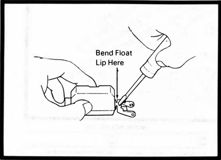
Bending Float Lip
