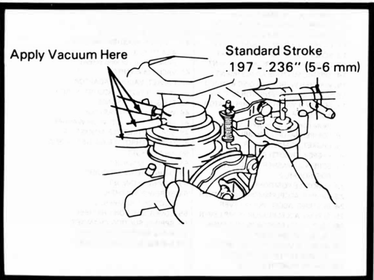
Checking Pump Stroke
